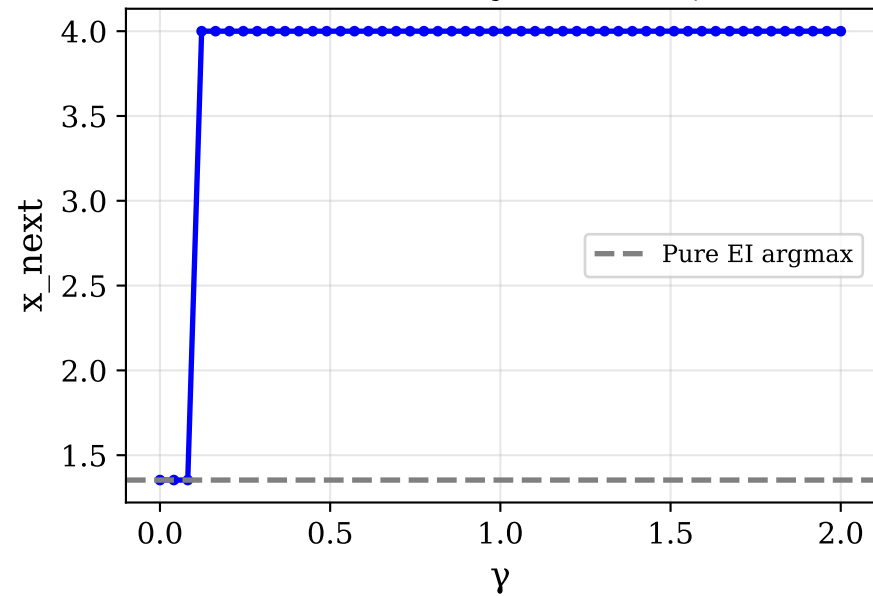
Next Query Point vs \gamma
