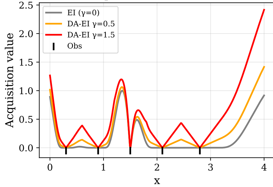
Acquisition: EI vs DA-EI
